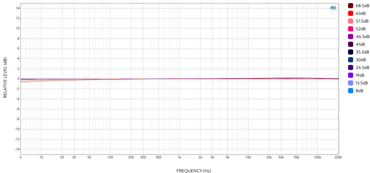
FREQUENCY RESPONSE: ALL GAIN SETTINGS
